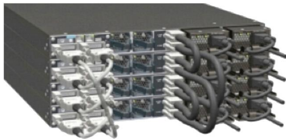
Figure 1. Cisco StackPower
